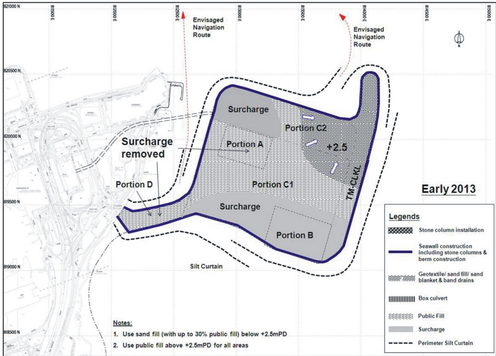
Figure 17 - Outline of Construction Sequence (Sheet 6 of 10)
